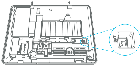
Figure 2: Battery connector
