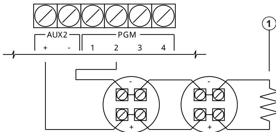
Figure 8: 2-wire smoke detector wiring
