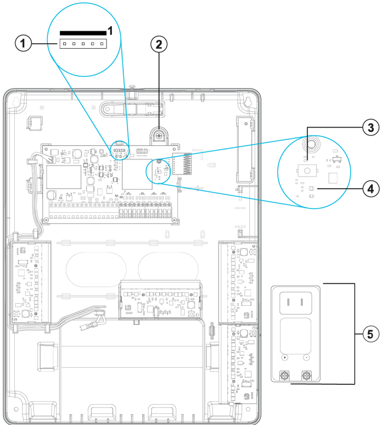
Figure 2: Mounting locations
